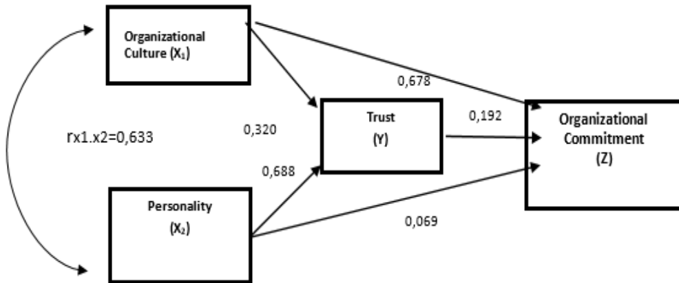
Fig. 2. Path Analysis of X 1 , X 2 , Y, and Z
