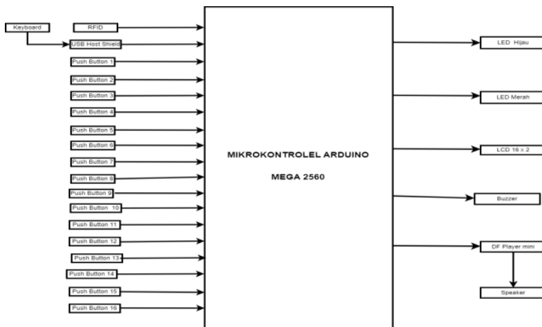
Gambar 11. Blok Diagram
